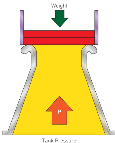
FIGURE 4-1 Weight Loaded Pressure Relief Valve
