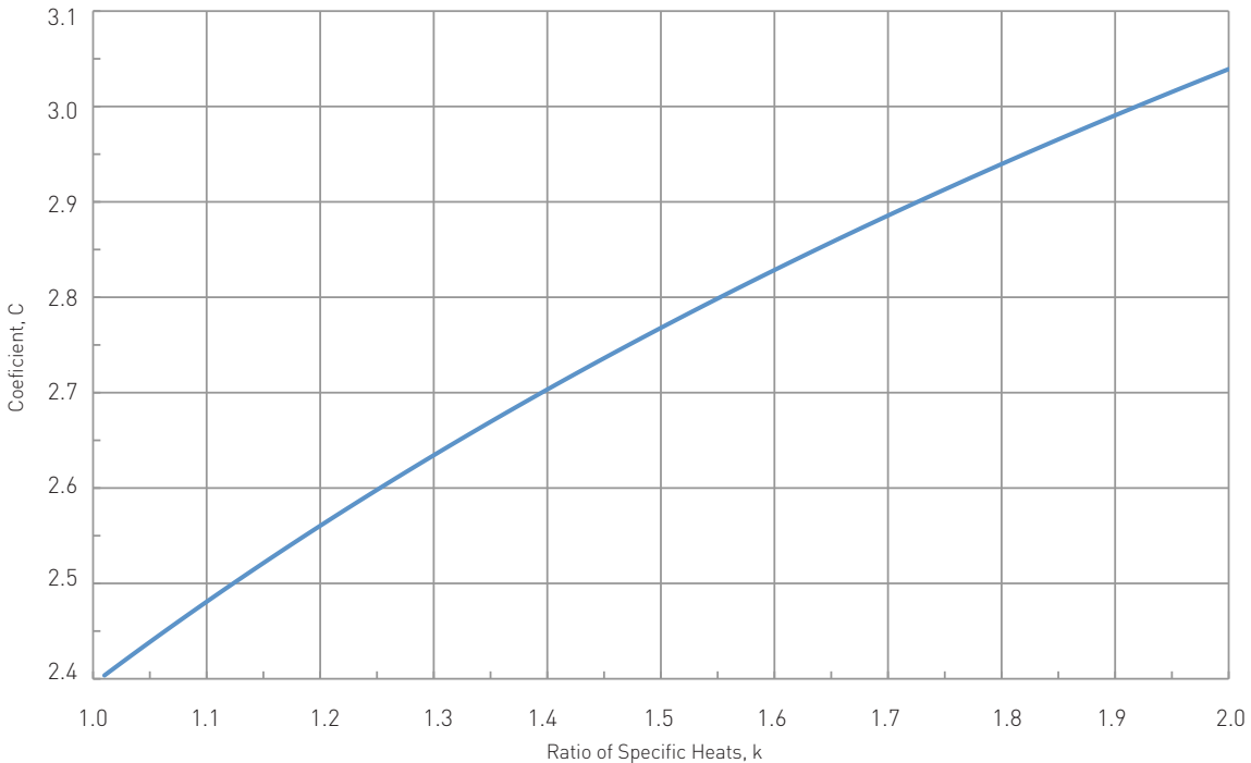
FIGURE 8-30 Gas Constant
