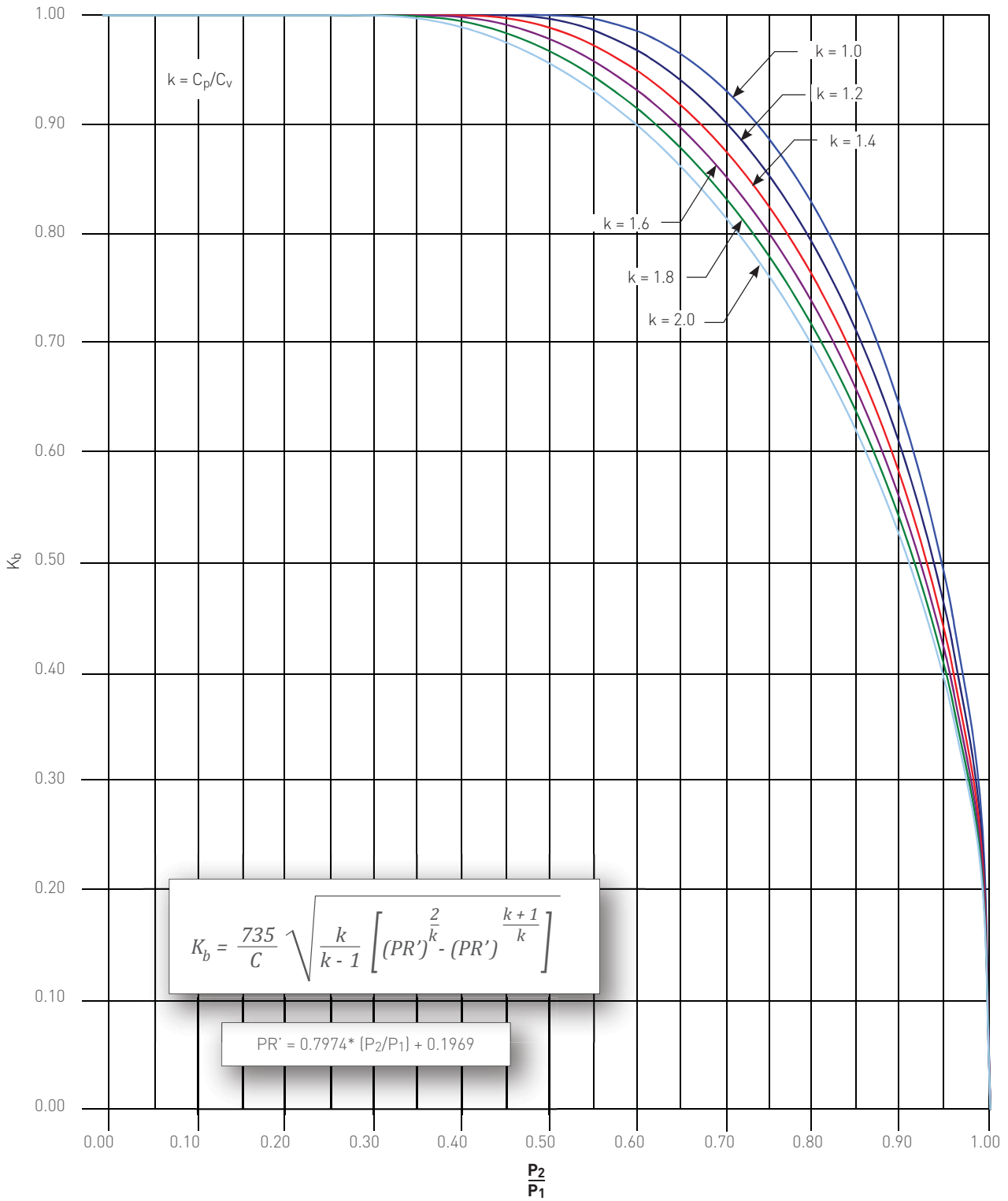
FIGURE 7-21 Anderson Greenwood Series 81P (-8 Orifice Only) Balanced Piston Direct Spring PRV Back Pressure Correction Factor ( K_b ) - Gas Service
