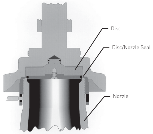
FIGURE 4-13 Metal Seated Direct Spring PRV
