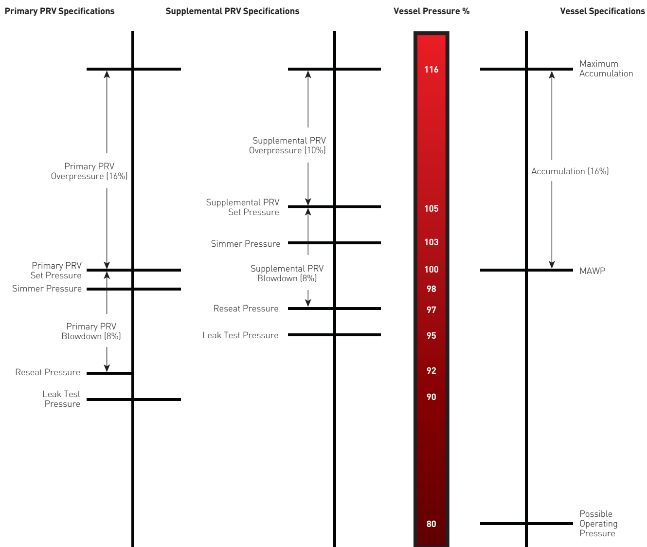
FIGURE 3-10 Typical Section VIII Multiple Valve (Non-Fire Case) Installation
