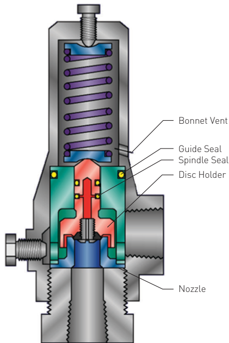
FIGURE 4-24 Balanced Piston Direct Spring PRV
